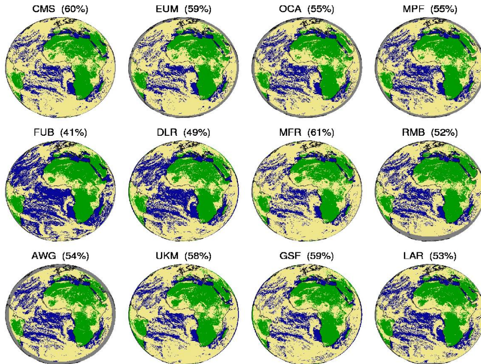
Figure 1: Cloud masks of the 12 CREW algorithms for 13-06-2008 at 12:00UTC.
