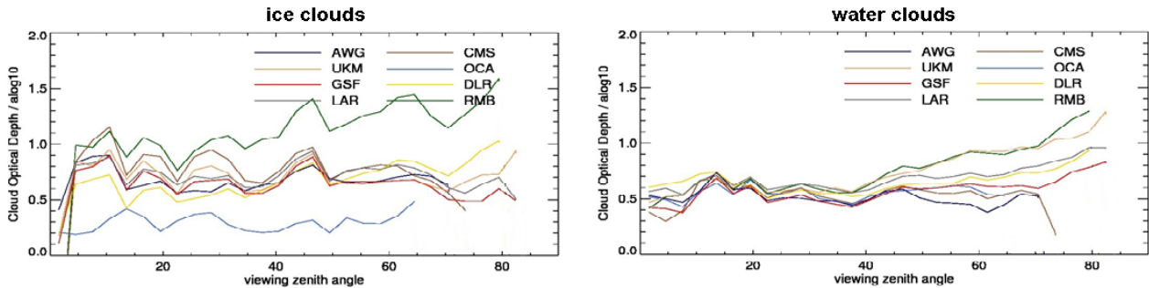
Figure 9: The left diagram shows the cloud optical depth of ice clouds in dependence of the viewing zenith angle for 13-06-2008, 12 UTC. The right diagram shows the same, but for water clouds.
