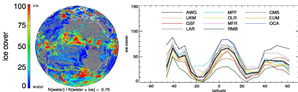
Figure 6: The left hand side shows the multi algorithm average of the cloud phase (water=0, unknown=50, ice=100). Light blue, green and yellow colors mark the areas were the multi algorithm ensemble can not certainly determine one cloud phase. The right hand side shows the zonal average for the individual algorithms, only pixels were every algorithm detected a cloud is taken into account (common cloud mask), both figures for for 13-06-2008 12 UTC.
